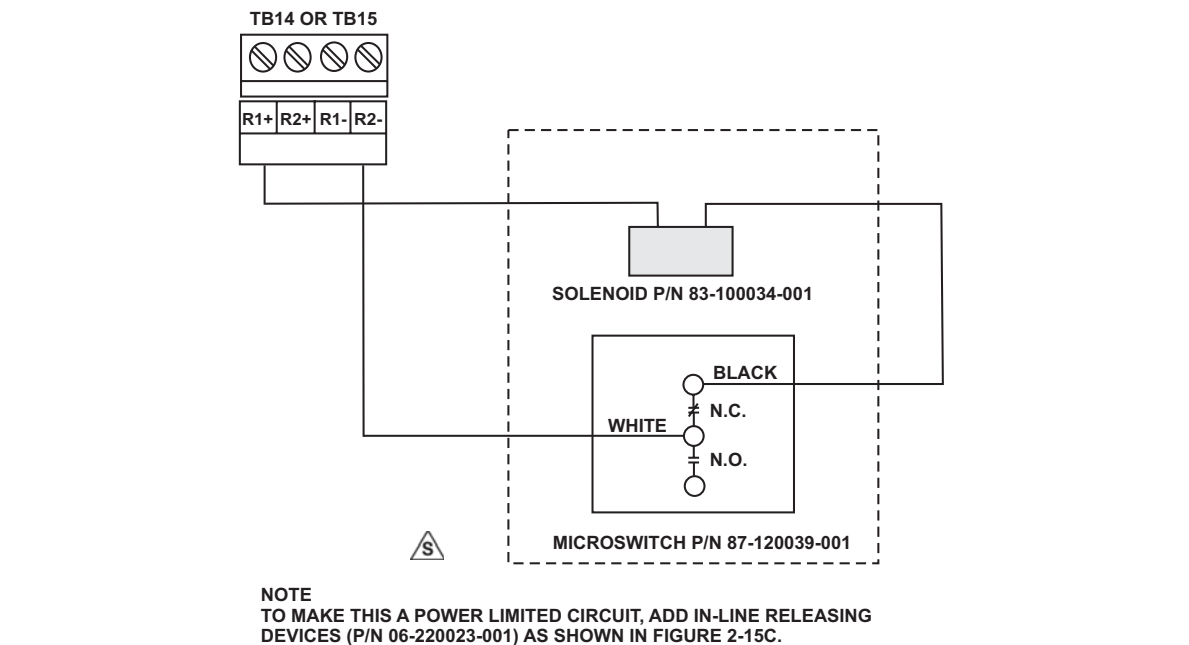
Figure 2-15E. Agent Release Circuit for XV and CXV Control Heads
