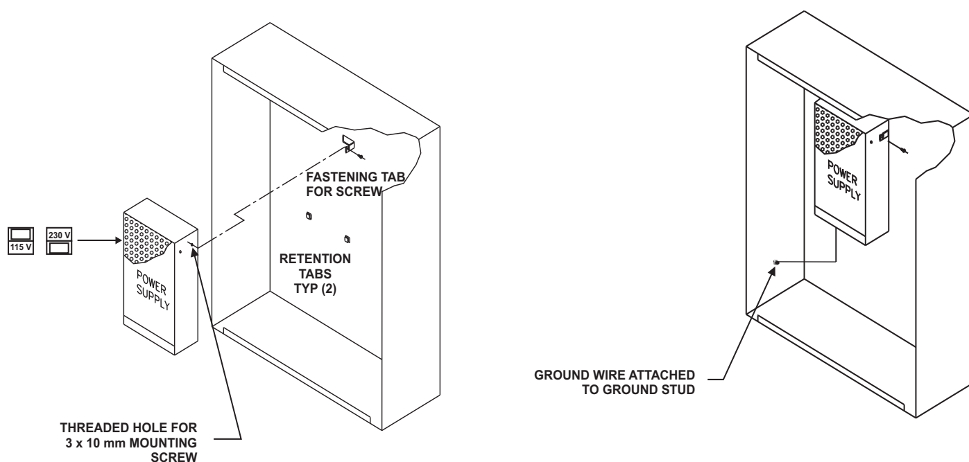
Figure 2-7. Power Supply Unit Installation
