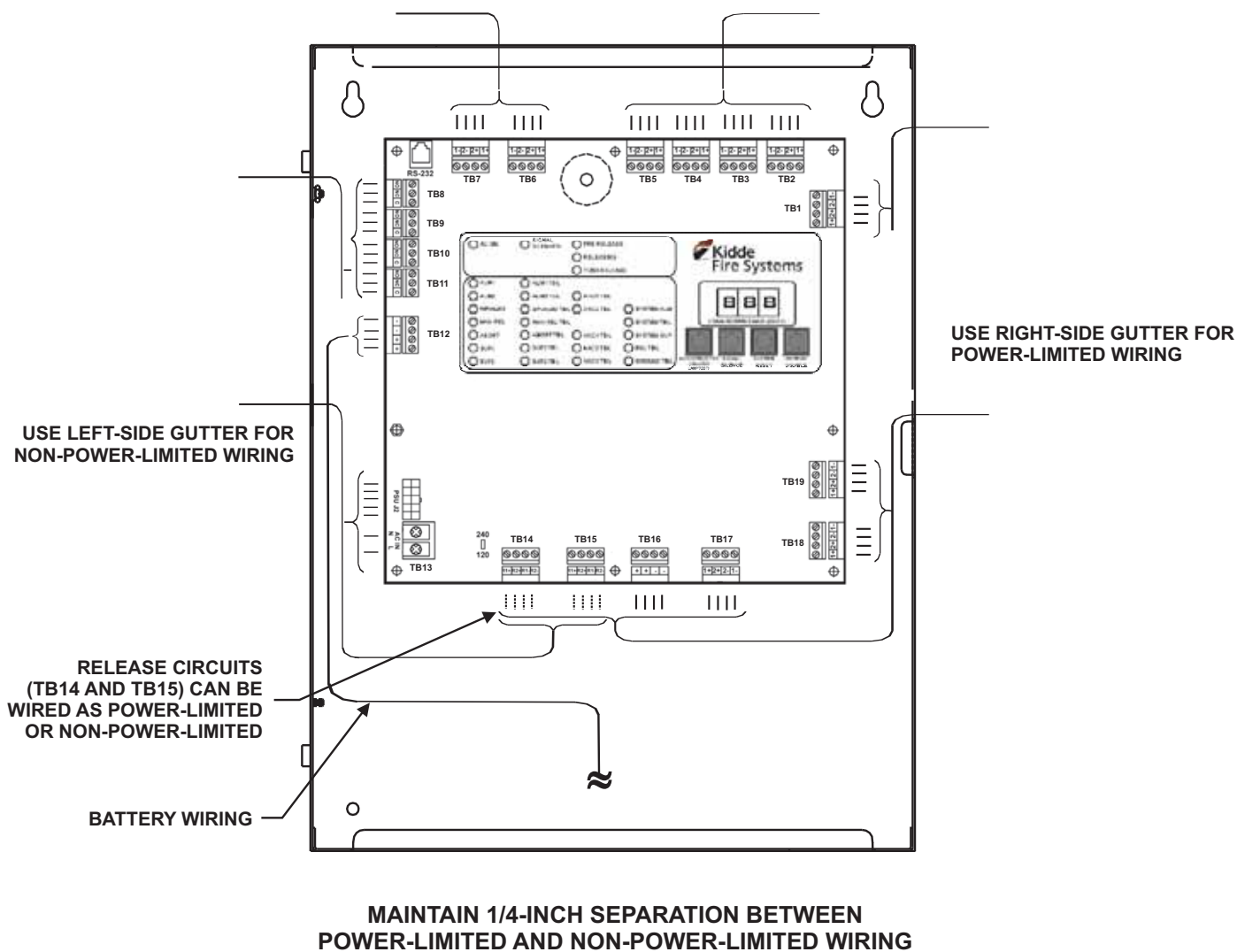
Figure F-1. Power-Limited and Non-Power-Limited Wiring
