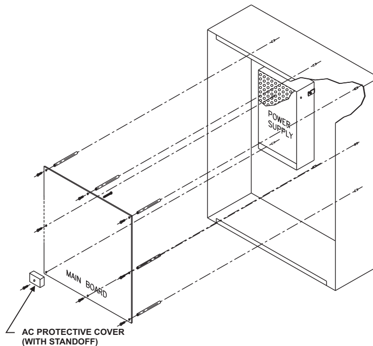
Figure 2-8. PCB Installation
