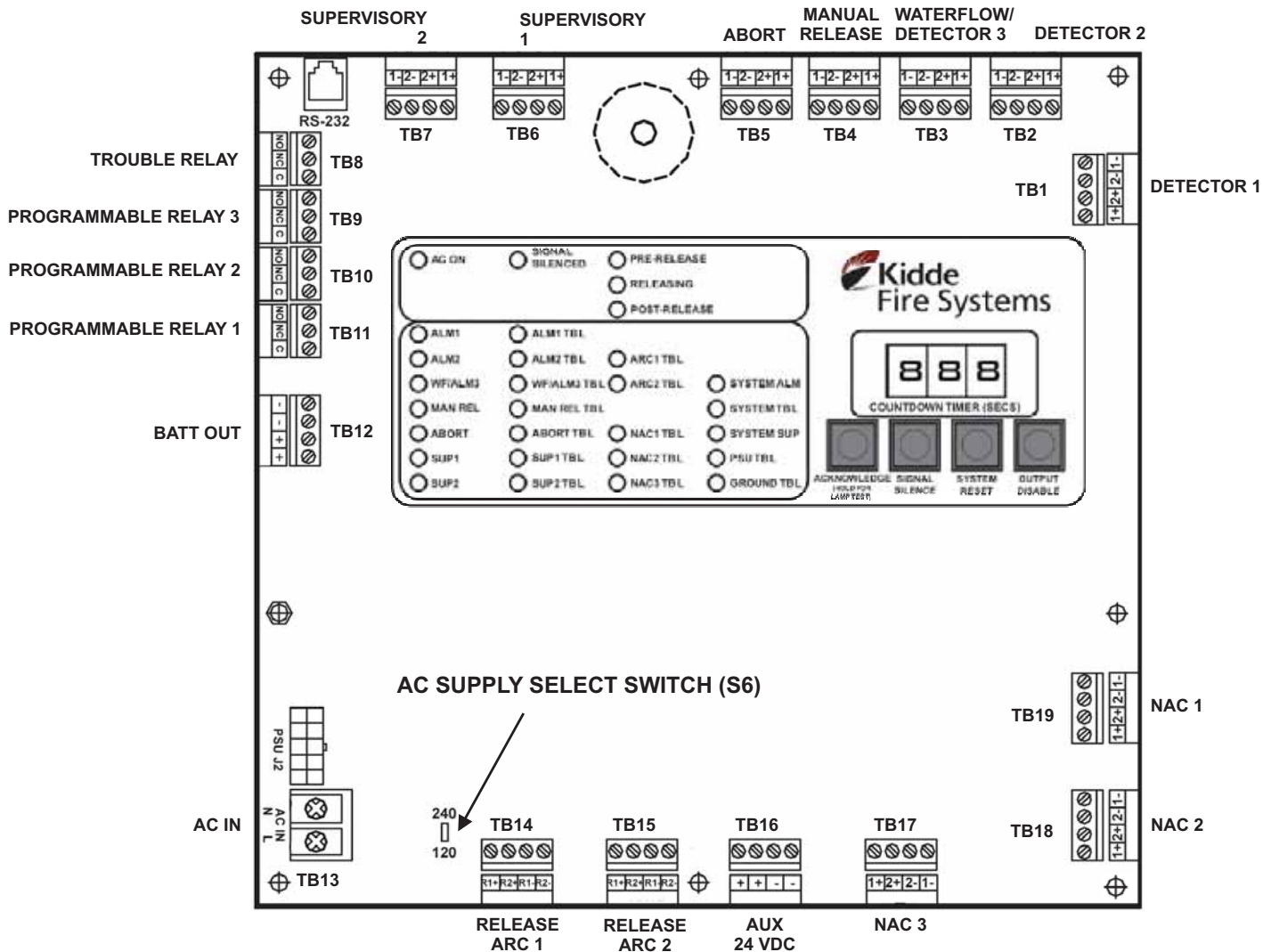
Figure 2-12. Printed Circuit Board
